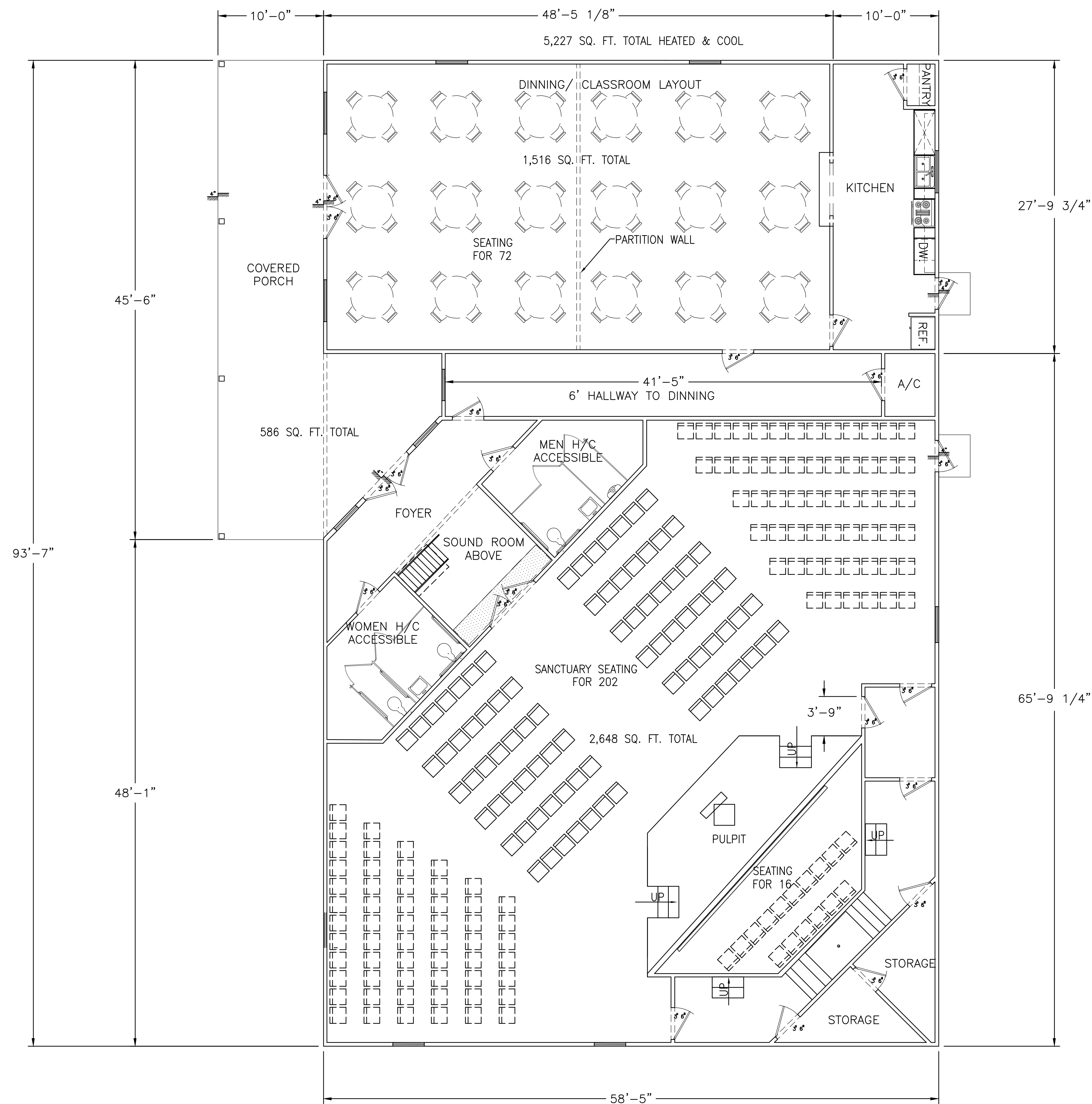
NEW FLOOR PLAN OPTION II
