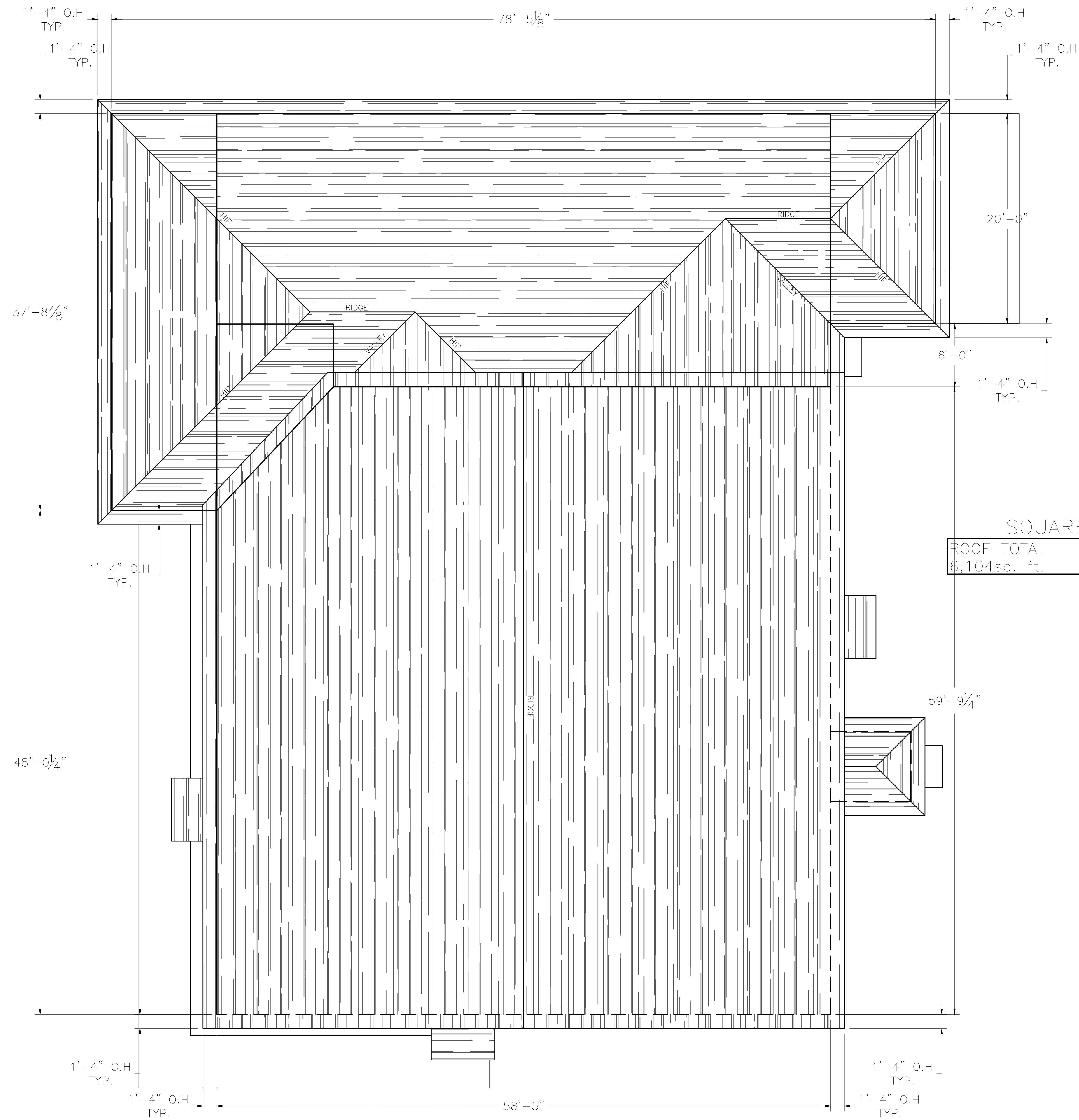
ROOFPLAN
