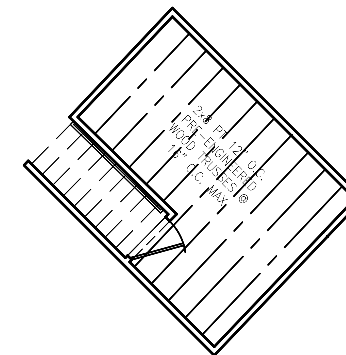
FRAMING PLAN
