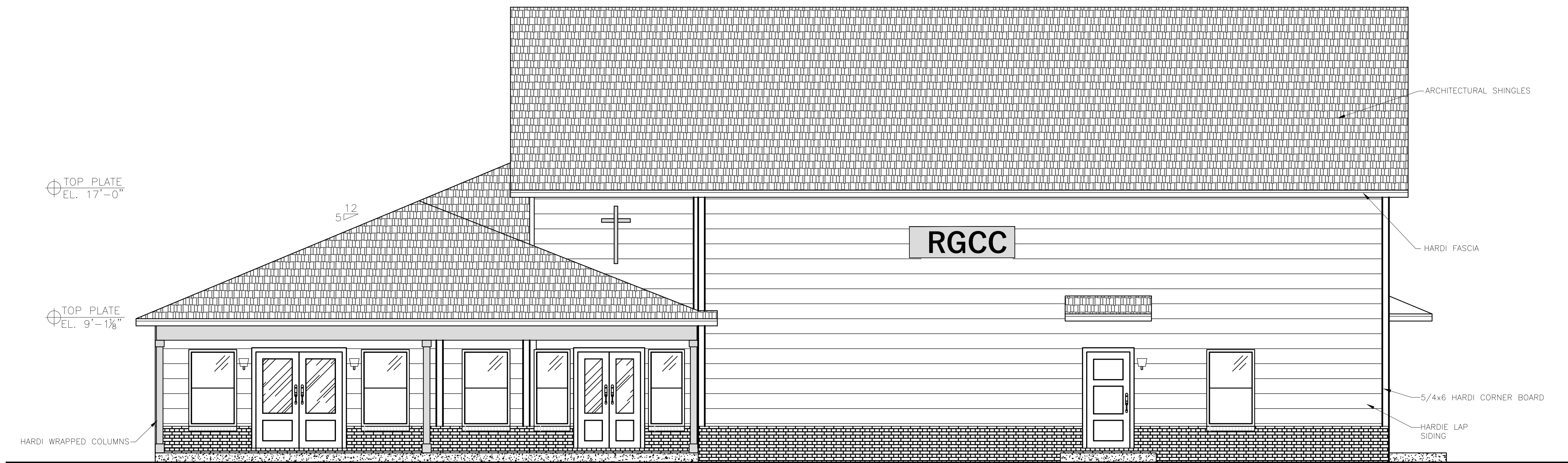
FRONT ELEVATION VIEW
