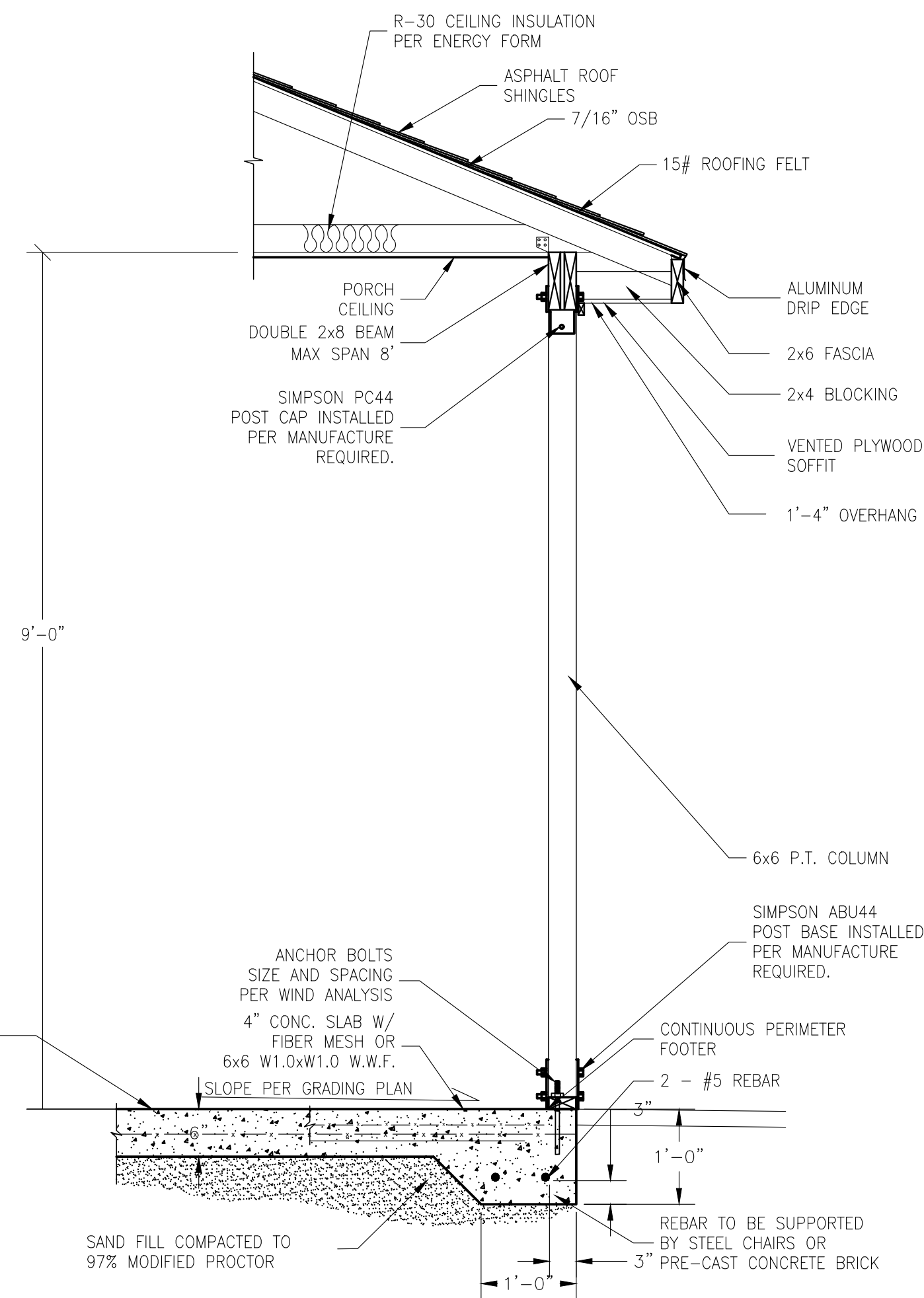
B POST DETAIL SCALE: 3/4"=1'-0"
