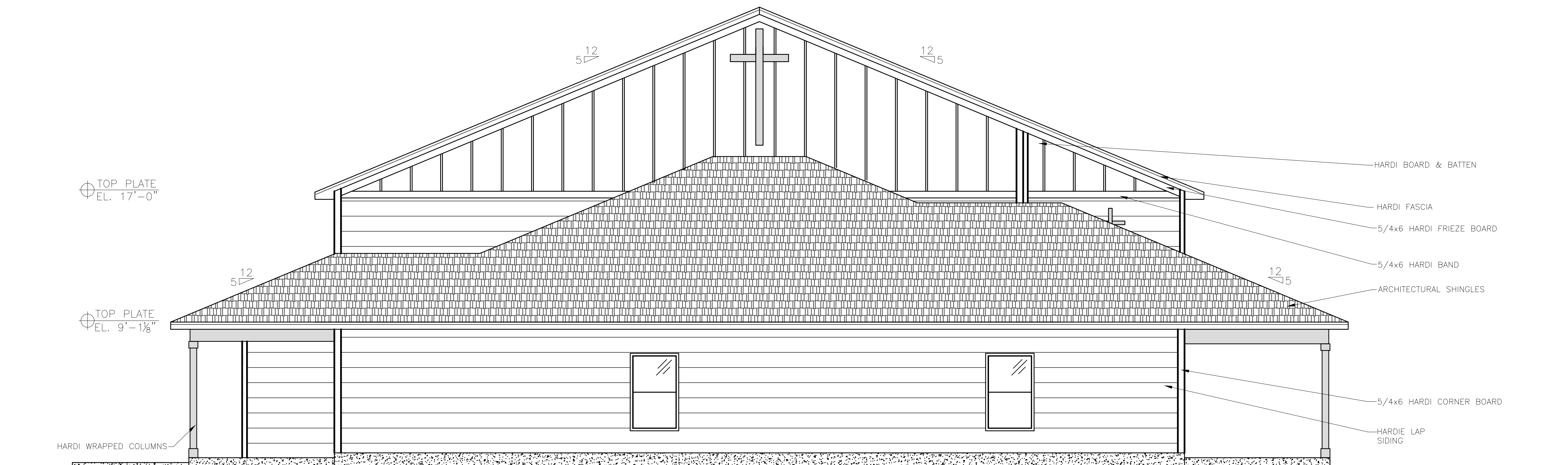
SIDE ELEVATION VIEW
