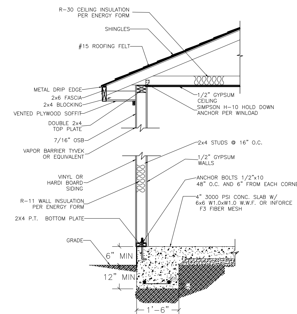
A WALL DETAIL SCALE: 3/4"=1'-0"
