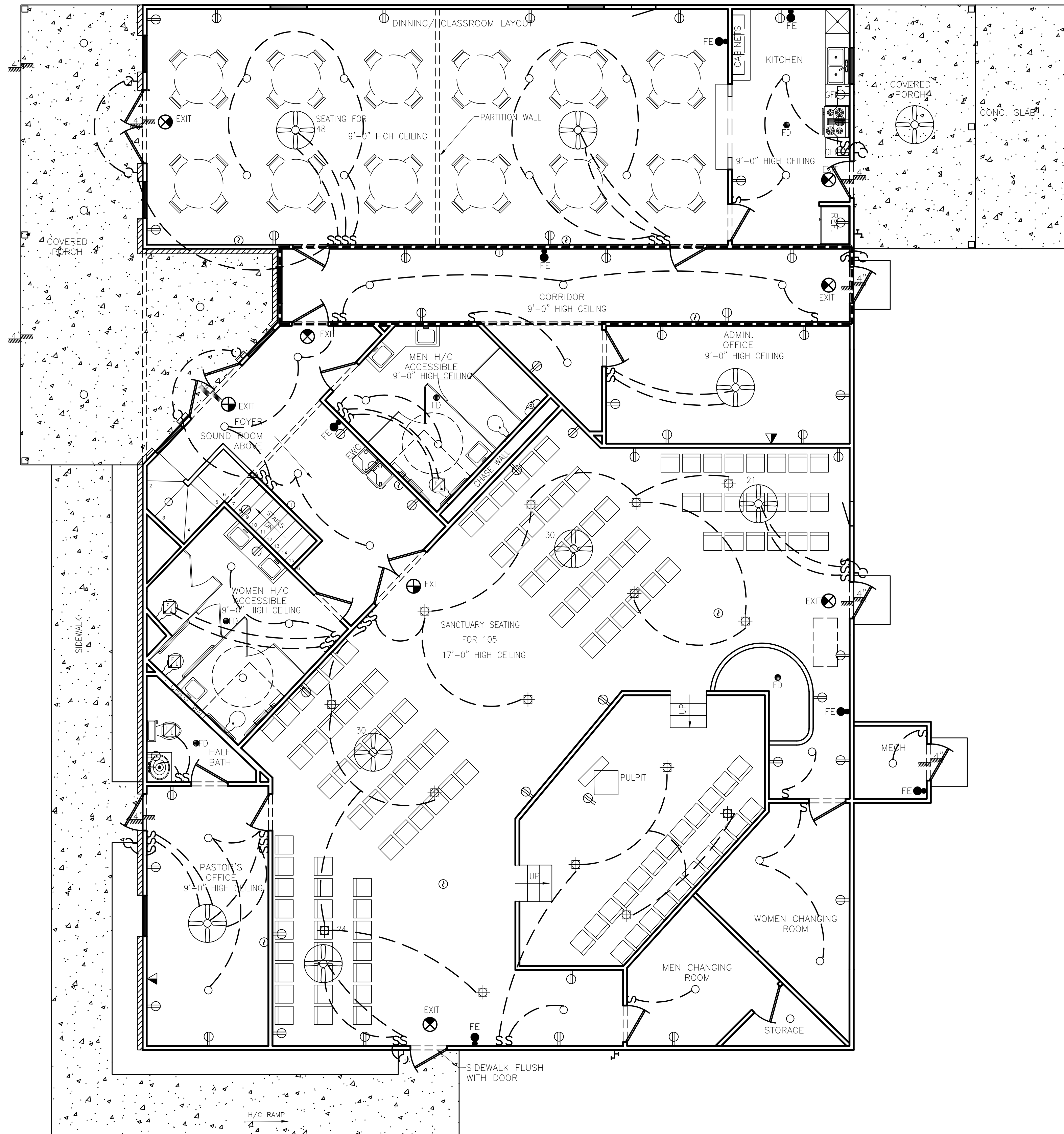
ELECTRICAL FLOOR PLAN
