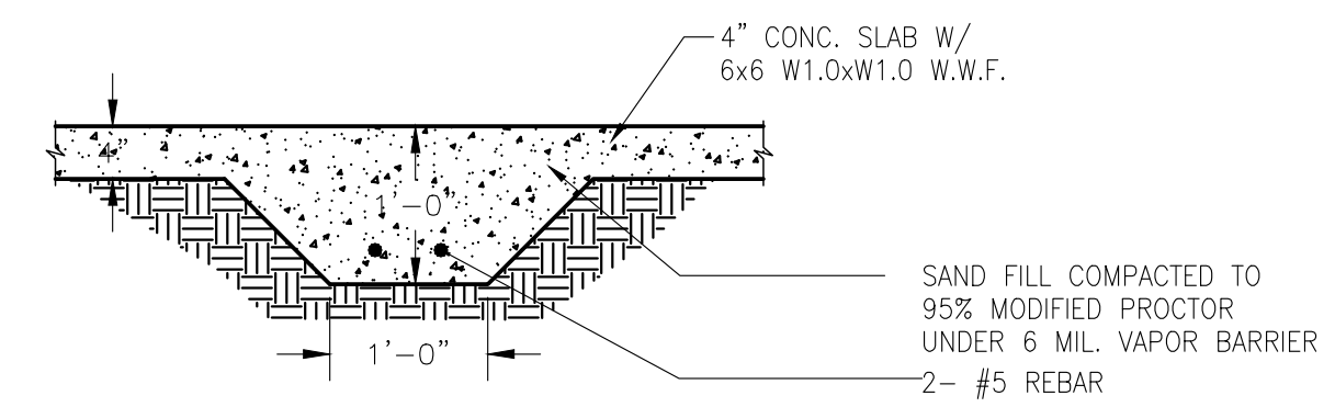
D INTERIOR DETAIL SCALE: 3/4"=1'-0"
