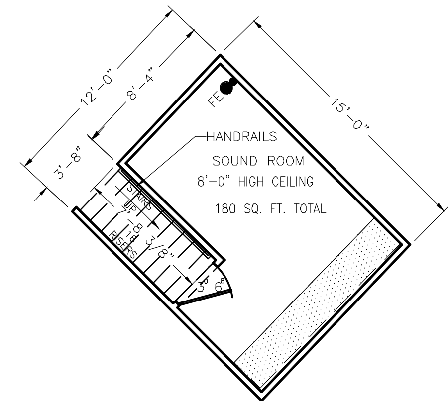
SOUND ROOM SCALE: 3/16"=1'-0"
