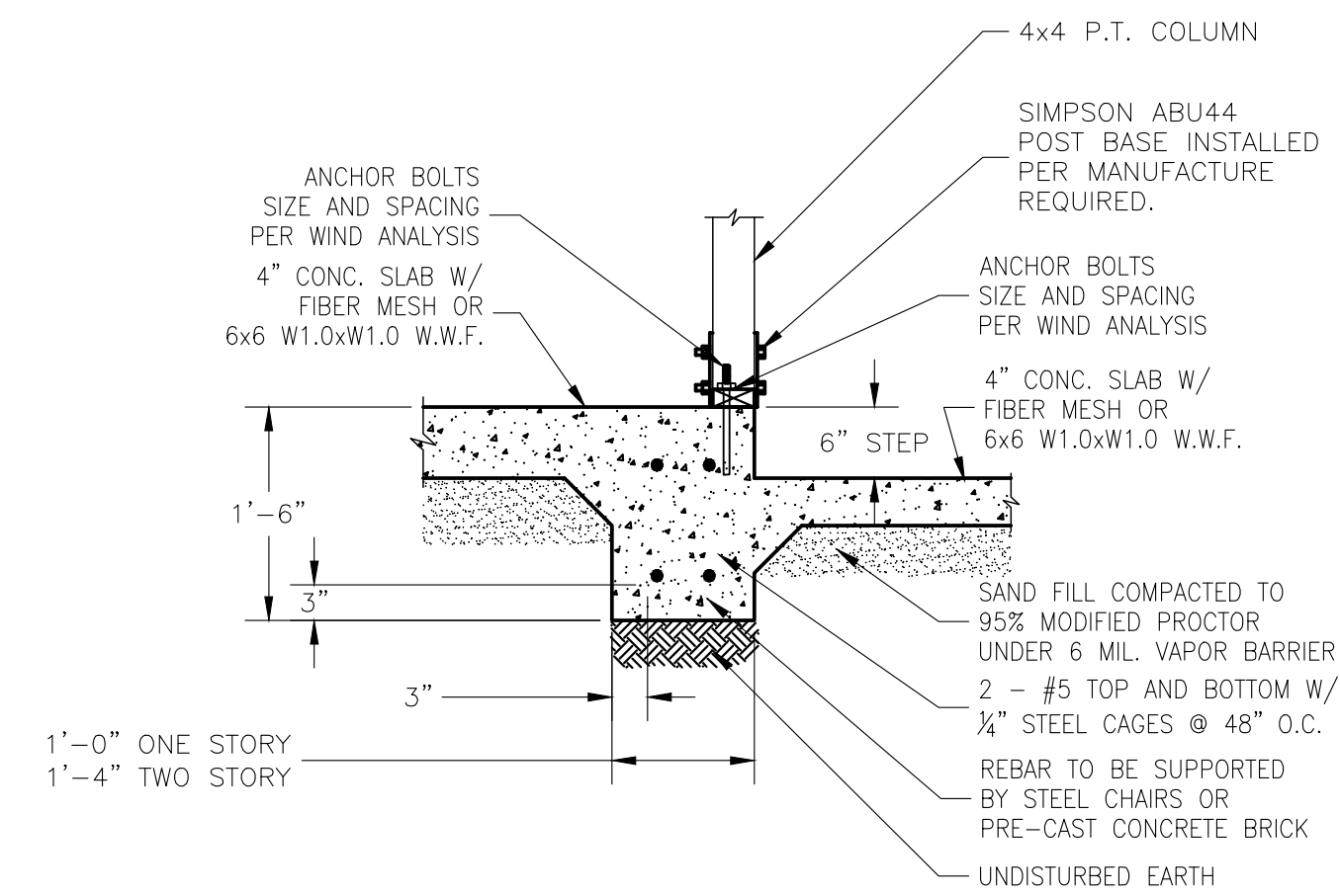
C PORCH STEPDOWN DETAIL SCALE: 3/4"=1'-0"
