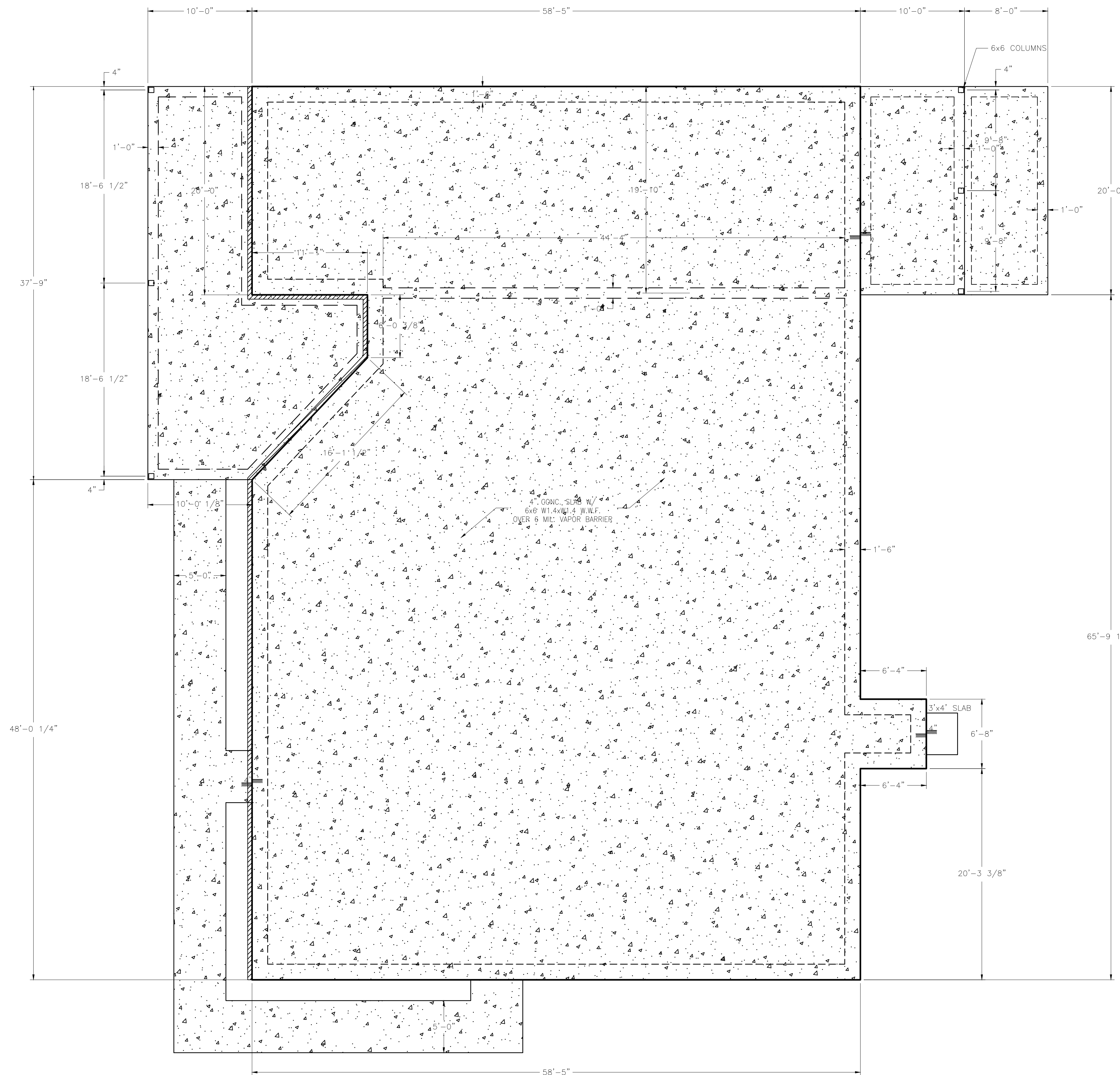
FOUNDATION PLAN
